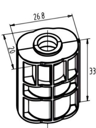
FCST-VBKB10 (12)
